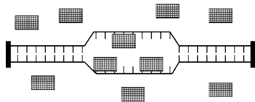
FIG. 1. Clamped DNA bubble in a region of size M , immersed in a bath of SSBs. SSBs do not bind across zippers.
