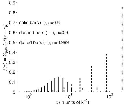
FIG. 3. Relaxation time spectrum for \sigma_0=10^{-3} and M=40 . For u=0.999 , the longest relaxation time dominates.
