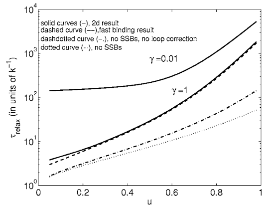
FIG. 5. Longest relaxation time as function of u , for \kappa=0.5 , \sigma_0=10^{-3} , M=20 , \lambda=5 .
