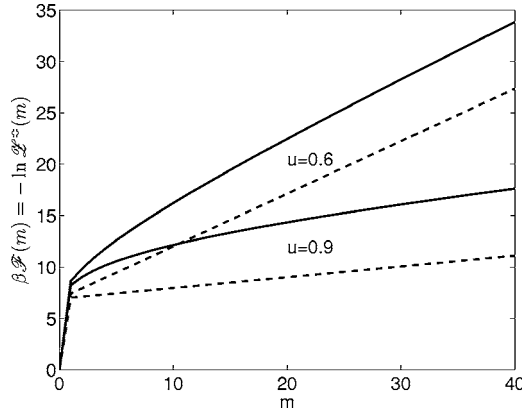
FIG. 2. Bubble free energy in absence of SSBs as function of bubble size m (solid line: c=1.76 ; dashed line: c=0 ). We chose \sigma_0=10^{-3} .
