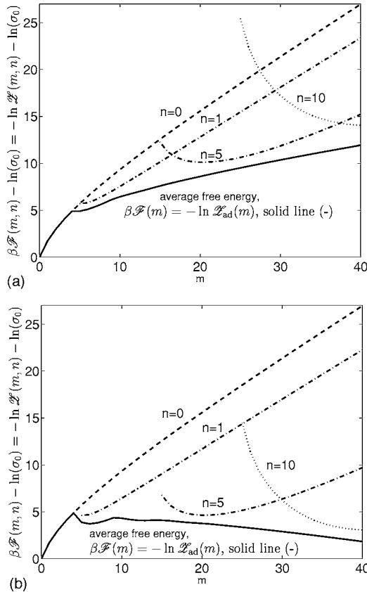
FIG. 4. Effective free energy in the limit \gamma \gg 1 (—), and free energy for various fixed n ( u=0.6 , M=40 , c=1.76 , \lambda=5 ). Top: \kappa=0.5 ; bottom: stronger binding, \kappa=1.5 .
